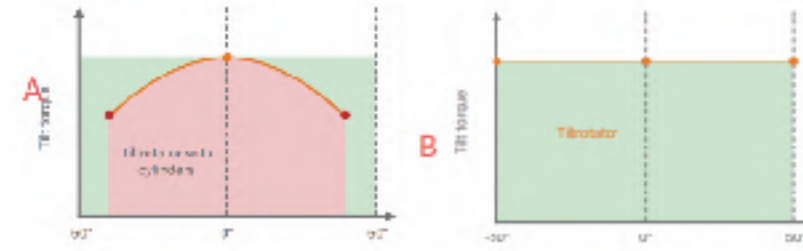
Comparison of output torque between cylinder and Tiltrotator.
